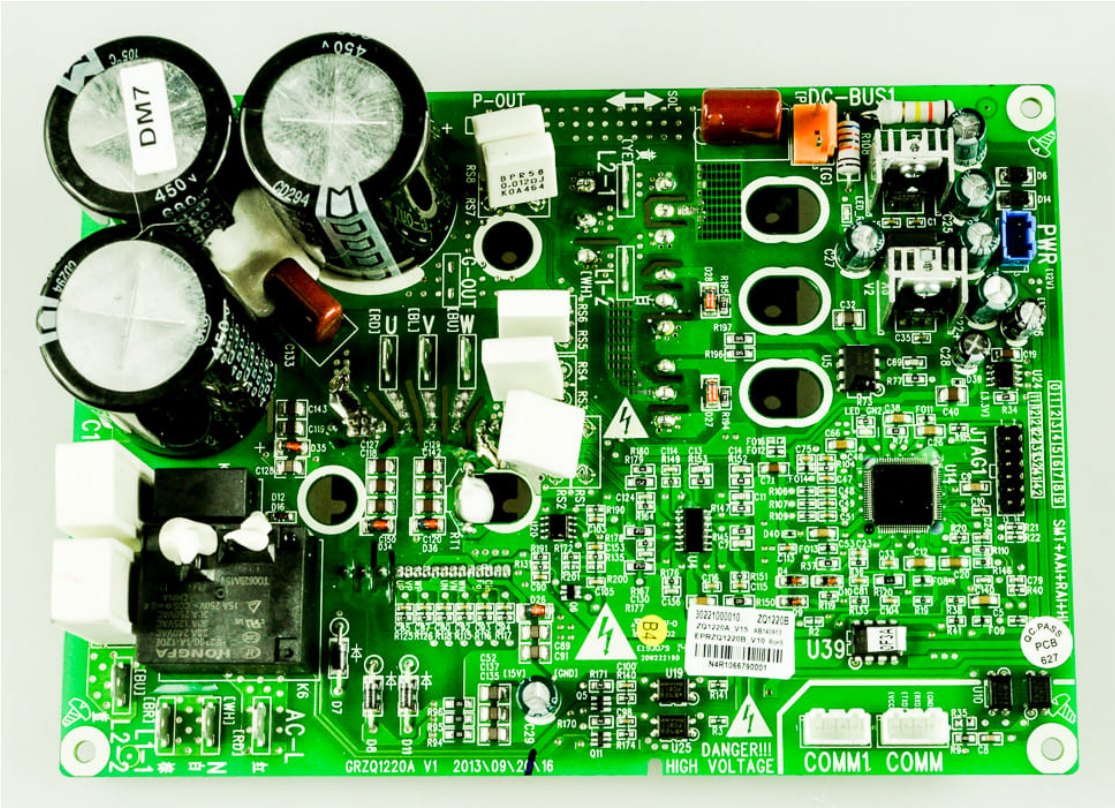
MAIN PCB 210901617AY
